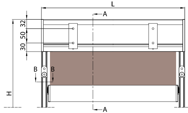
Guida a parete - Wall guide - Coulisse façade - Wandführung
