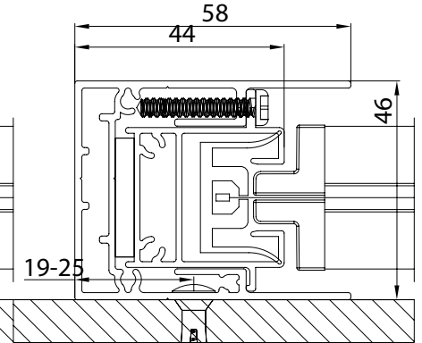
Guida a parete - Wall guide Coulisse façade - Wandführung B-B
