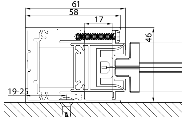
Guida a parete - Wall guide Coulisse façade - Wandführung B-B
