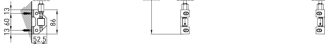
Supporto a nicchia - Niche support - Support tableau - Nischenkonsole
