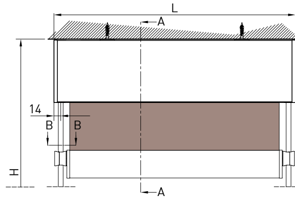
Supporto a parete - Wall support - Support au mur - Wandkonsole
