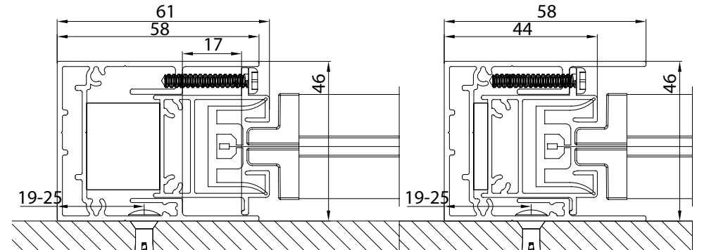
Guida a parete - Wall guide Coulisse façade - Wandführung B-B
