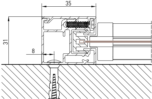
Guida a parete - Wall guide Coulisse façade - Wandführung
