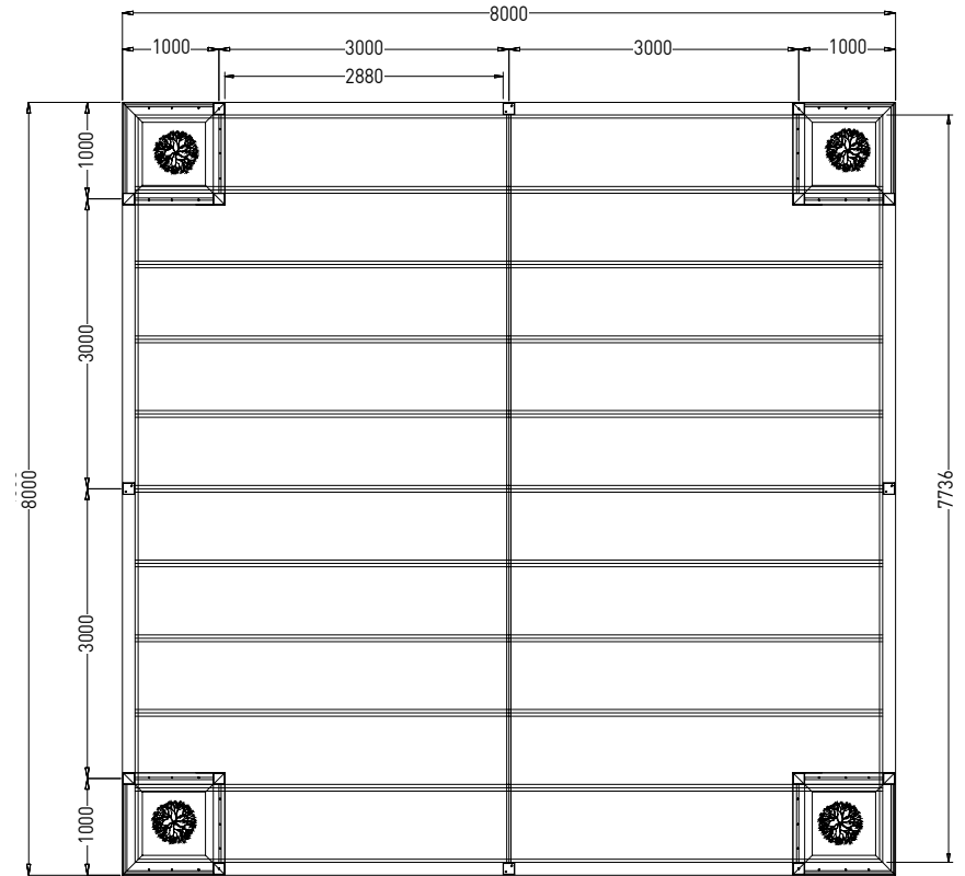
VISTA IN PIANTA / PLAN VIEW
